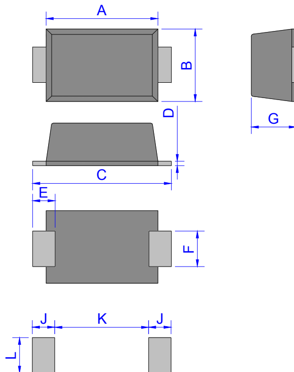
SOD-123FL
